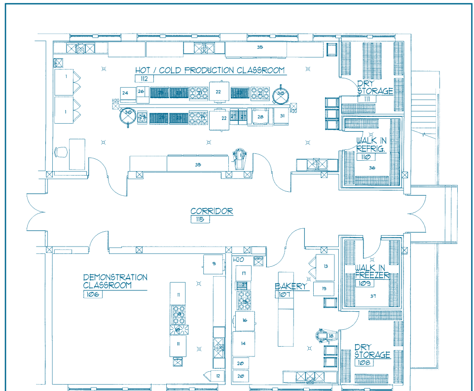
CULINARY ARTS WING - PHASE 6 - 3724 SF
